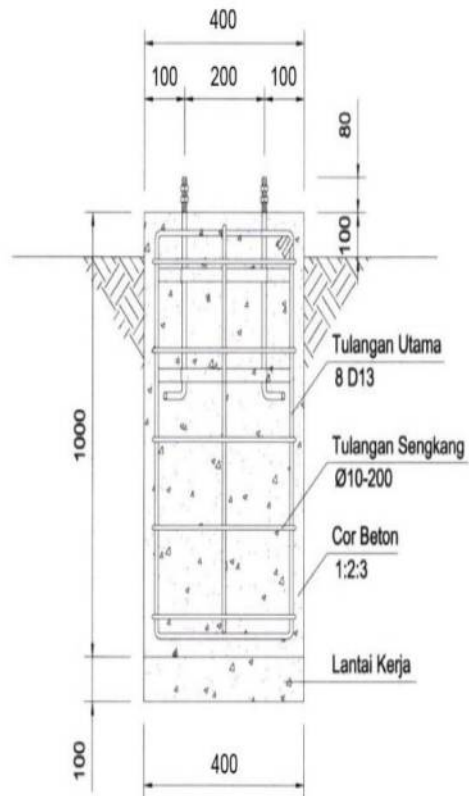
TAMPAK SAMPIING
