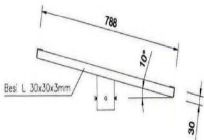
TAMPAK SAMPING
