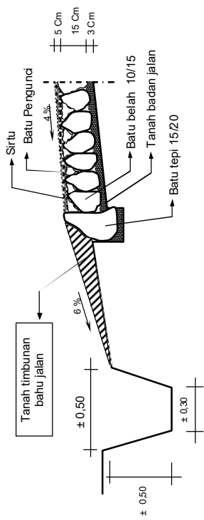
DETAIL POT. MELINTANG
